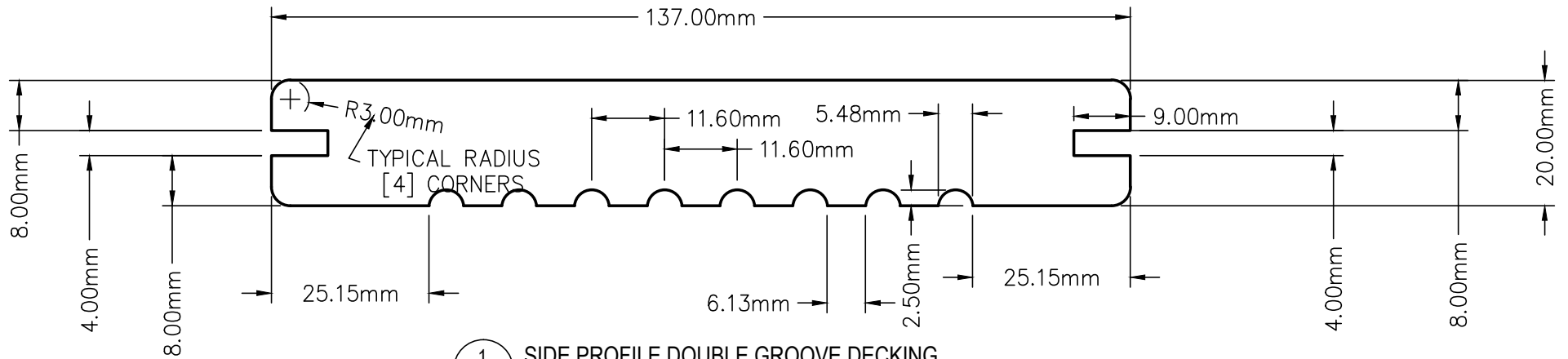
1 SIDE PROFILE DOUBLE GROOVE DECKING 01 SCALE 1:1
